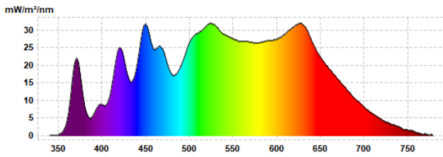
Spektrum DLS Color Viewing Light D50
