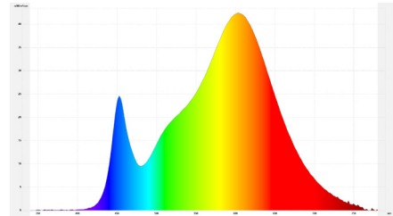
Spektrum DLS Color Viewing Light CIE B2
